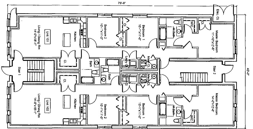
1st Floor Plan Scale: n.l.s.
