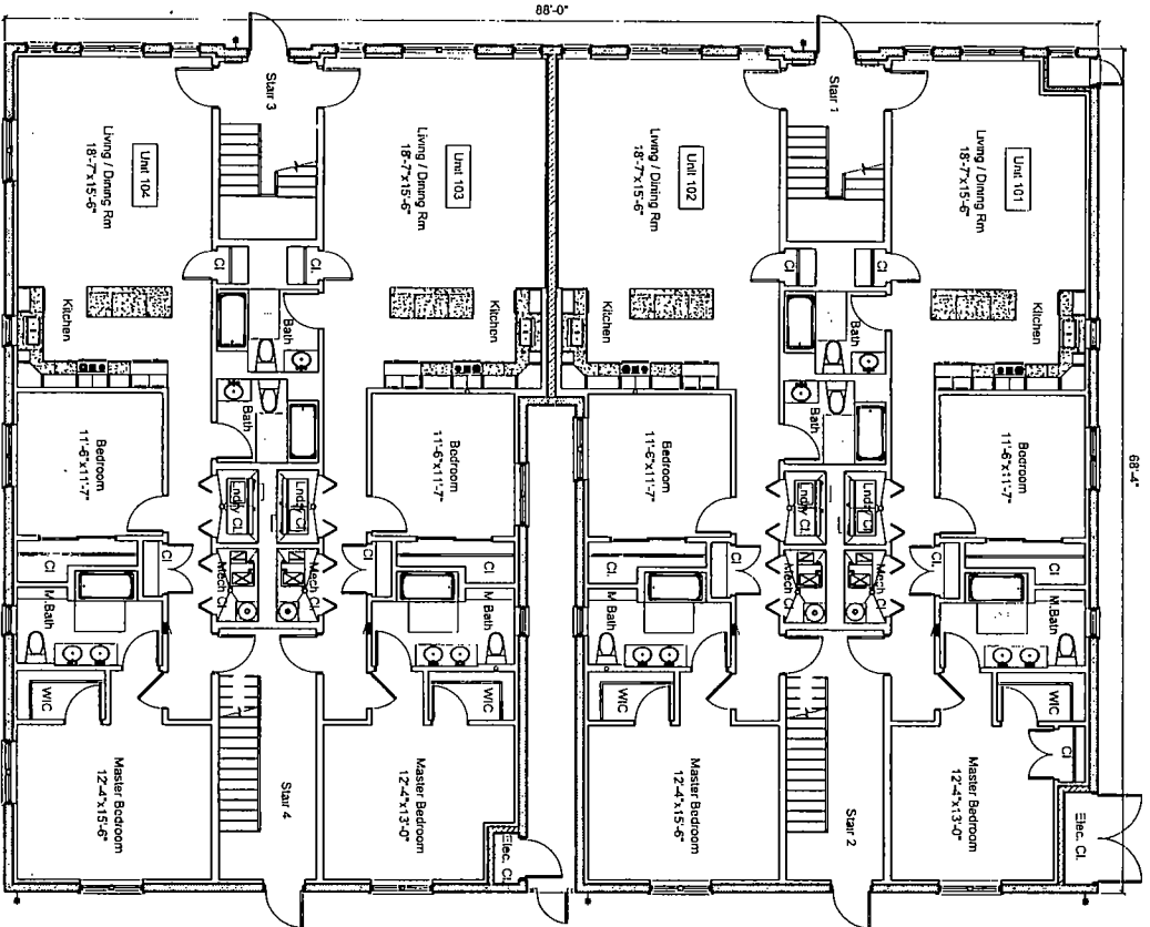
1st Floor Plan Scale: n.l.s.
