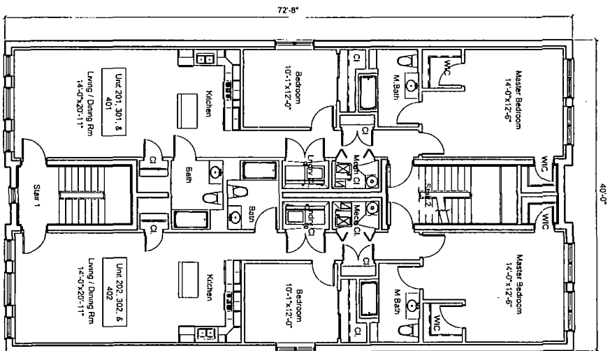
2nd, 3rd, & 4th Floor Plan
