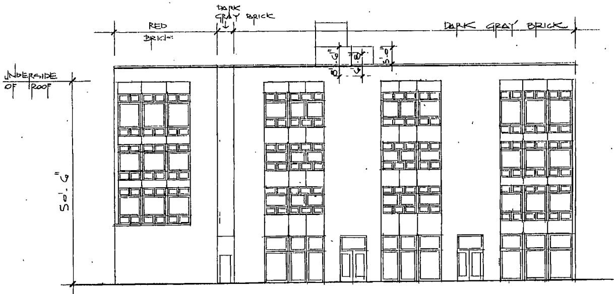
ARMITAGE ELEVATION 1/8" = 1'-0"
